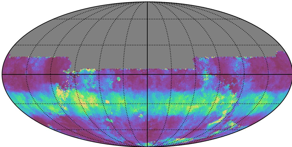
extra_ss_neo3_v3.4_10yrs All sky u band: Median normairmass
