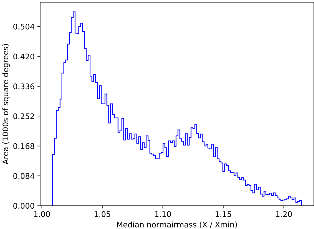
extra_ss_neo3_v3.4_10yrs All sky u band: Median normairmass
