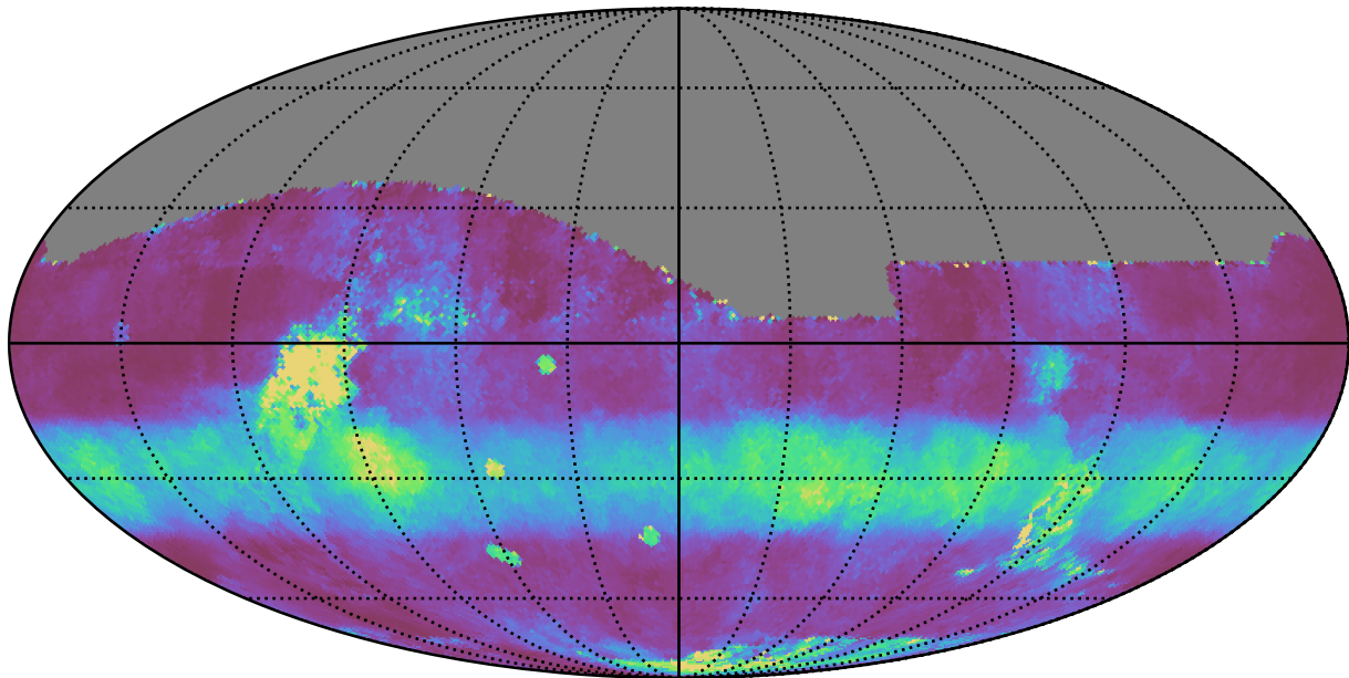
extra_ss_neo3_v3.4_10yrs All sky r band: Median normairmass
