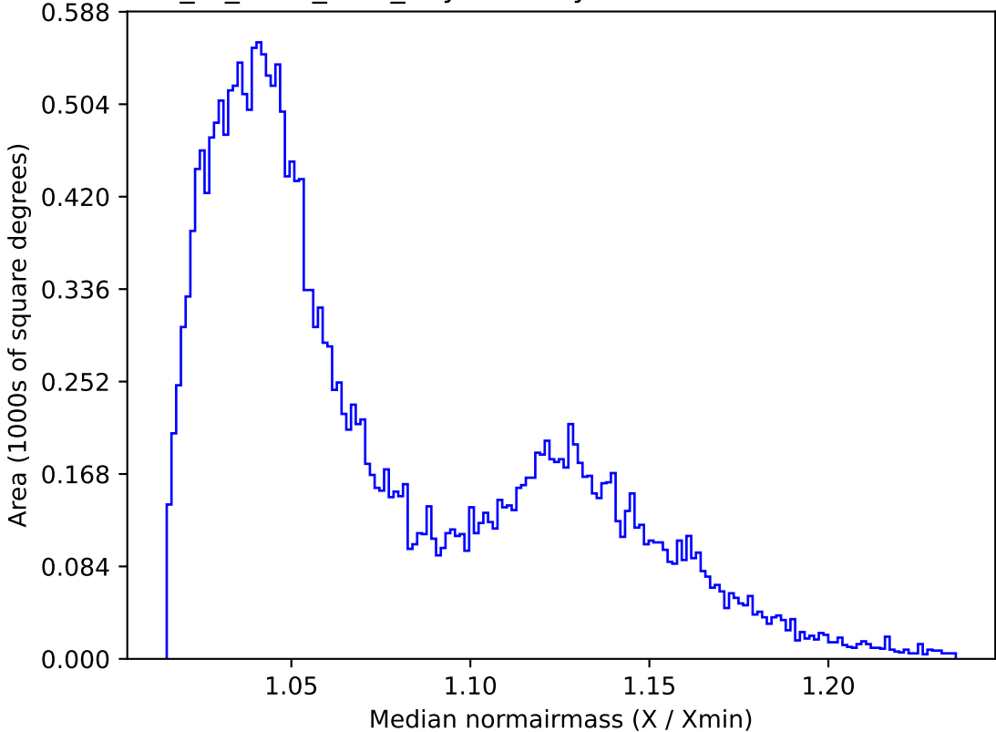
extra_ss_neo3_v3.4_10yrs All sky r band: Median normairmass
