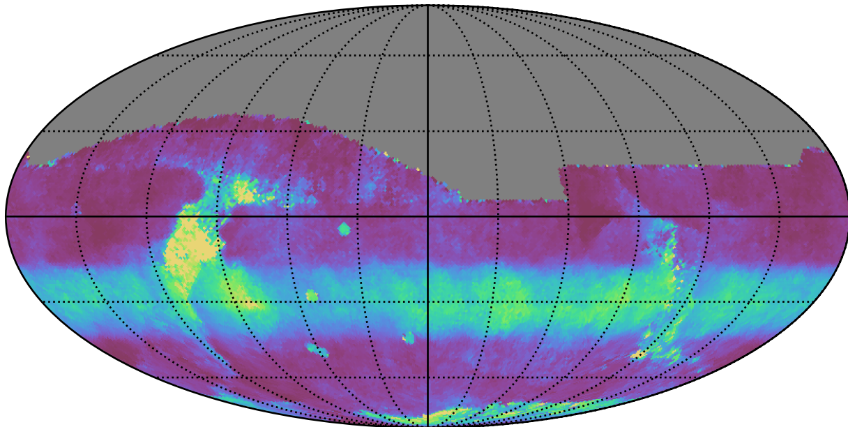
extra_ss_neo3_v3.4_10yrs All sky i band: Median normairmass
