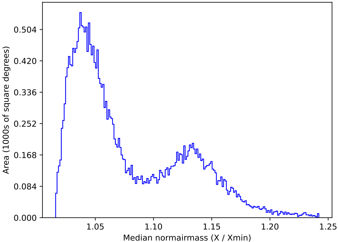
extra_ss_neo3_v3.4_10yrs All sky i band: Median normairmass
