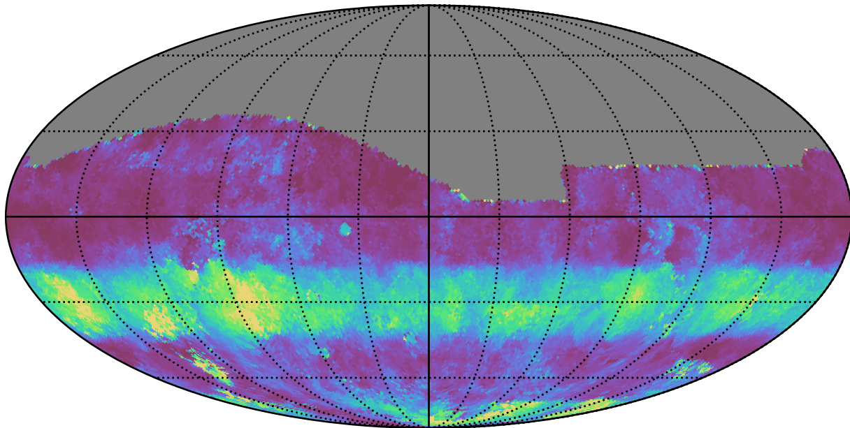
extra_ss_neo3_v3.4_10yrs All sky g band: Median normairmass
