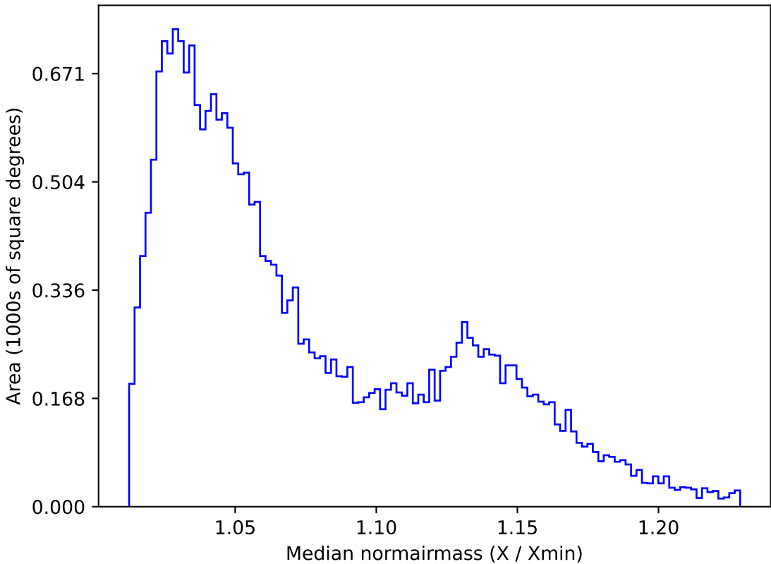
extra_ss_neo3_v3.4_10yrs All sky g band: Median normairmass
