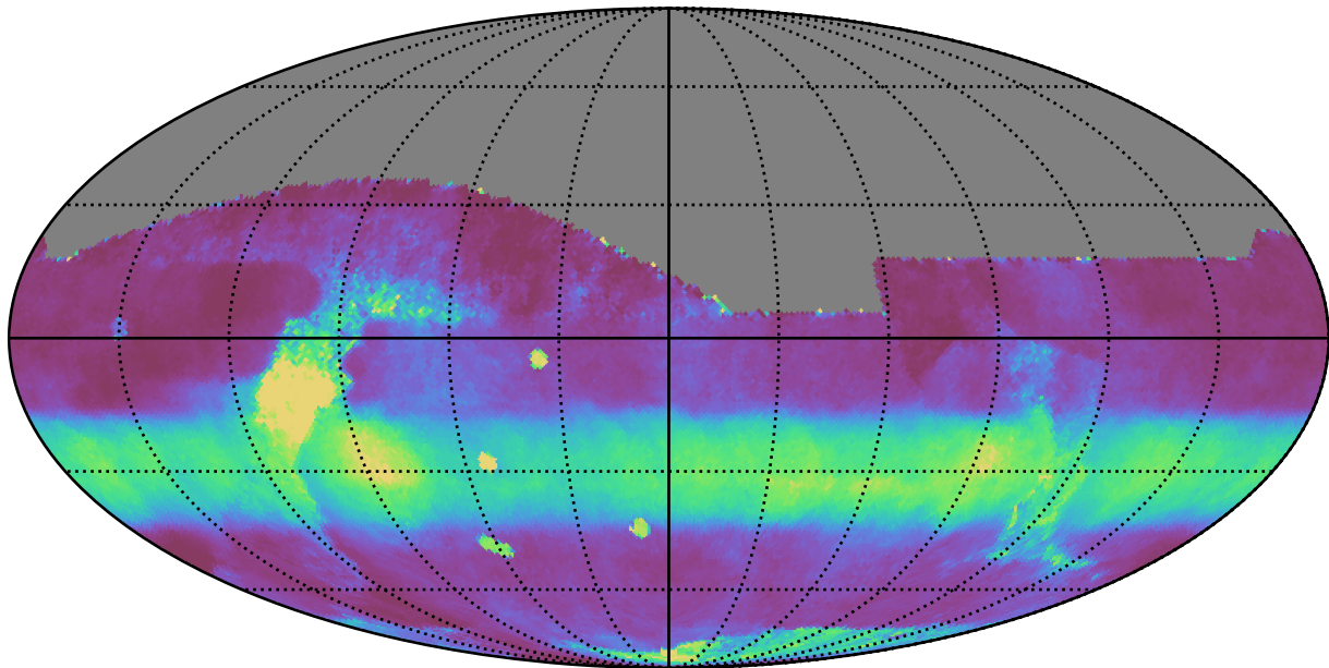
extra_ss_neo3_v3.4_10yrs All sky all bands: Median normairmass
