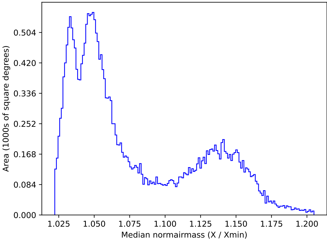
extra_ss_neo3_v3.4_10yrs All sky all bands: Median normairmass
