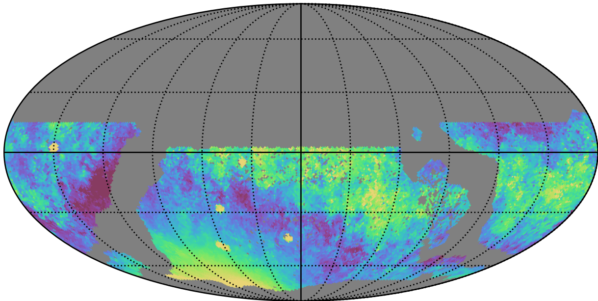
extra_ss_neo3_v3.4_10yrs WFD z band: Median moonDistance
