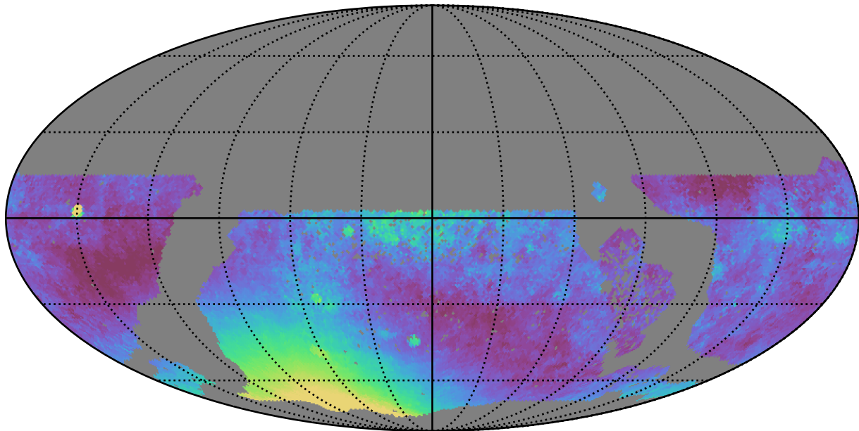
extra_ss_neo3_v3.4_10yrs WFD y band: Median moonDistance
