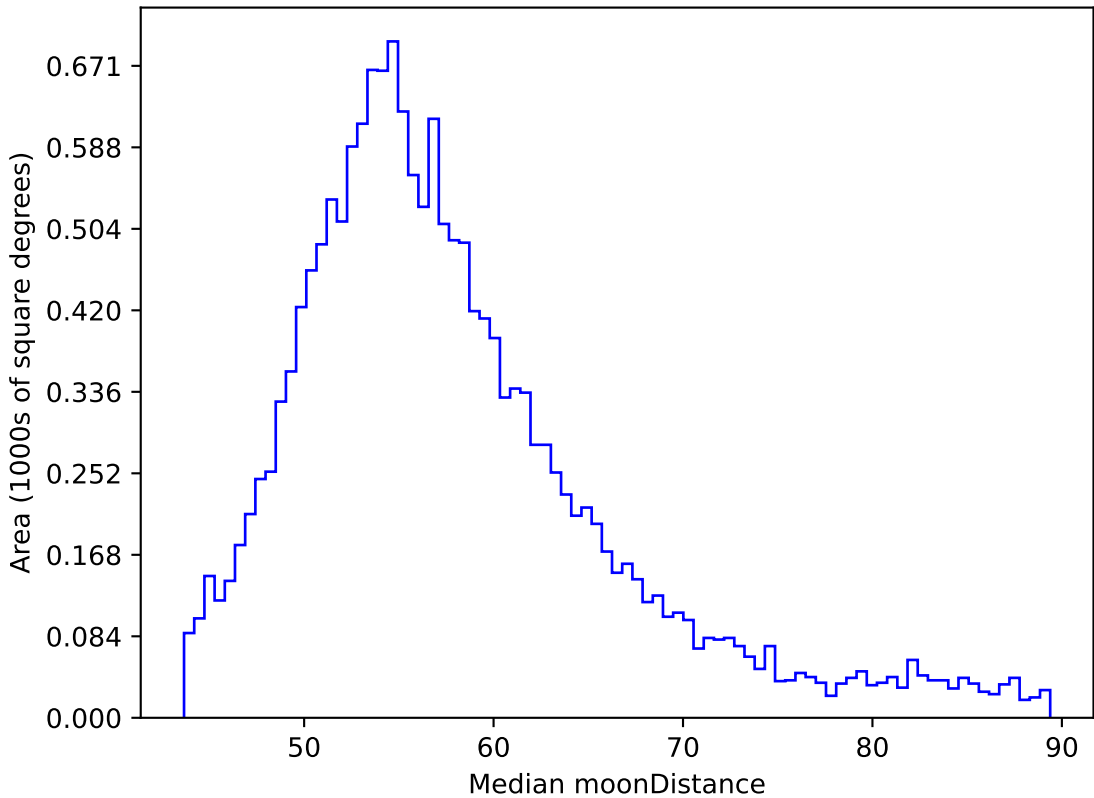
extra_ss_neo3_v3.4_10yrs WFD y band: Median moonDistance
