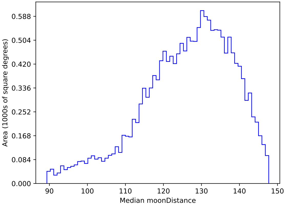
extra_ss_neo3_v3.4_10yrs WFD u band: Median moonDistance
