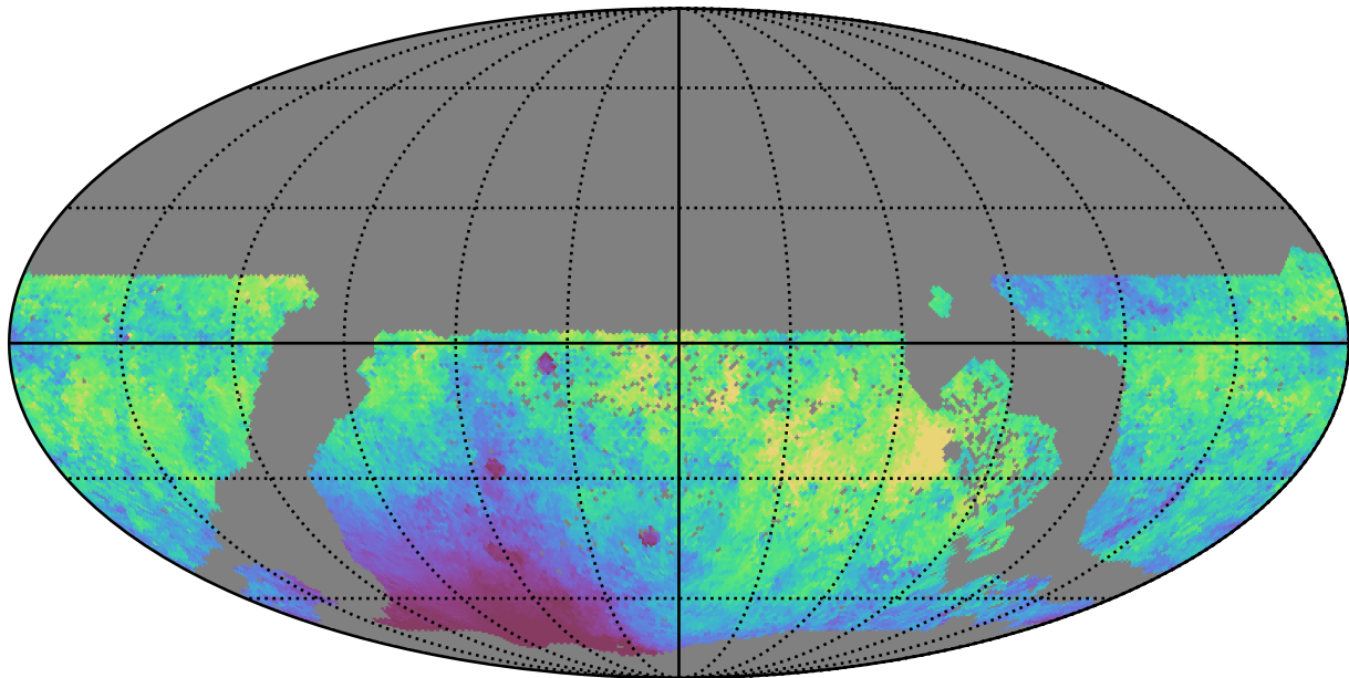
extra_ss_neo3_v3.4_10yrs WFD r band: Median moonDistance
