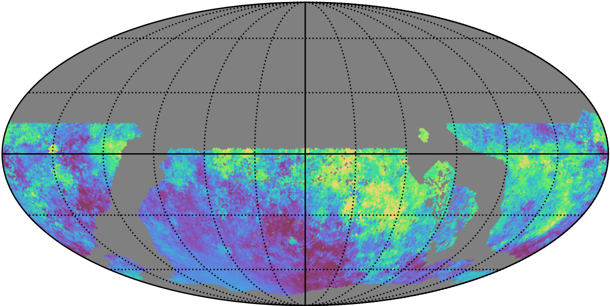
extra_ss_neo3_v3.4_10yrs WFD i band: Median moonDistance
