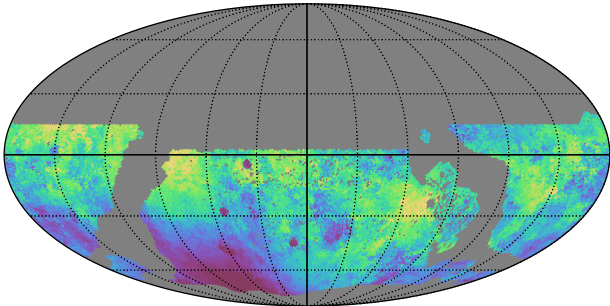
extra_ss_neo3_v3.4_10yrs WFD g band: Median moonDistance
