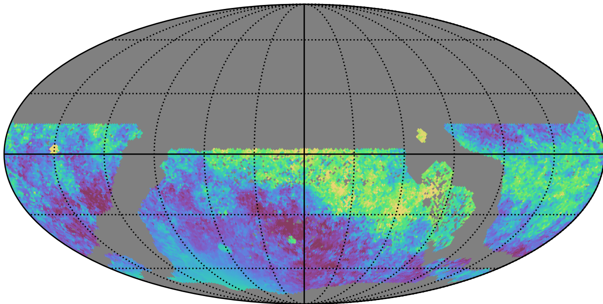
extra_ss_neo3_v3.4_10yrs WFD all bands: Median moonDistance
