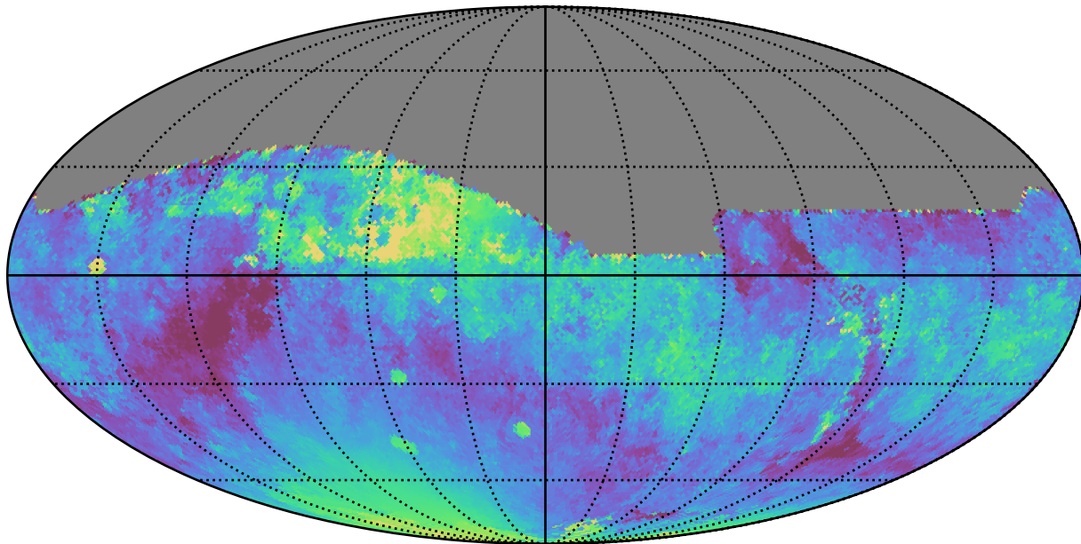
extra_ss_neo3_v3.4_10yrs All sky z band: Median moonDistance
