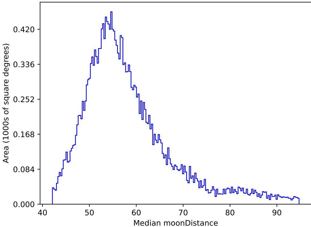
extra_ss_neo3_v3.4_10yrs All sky y band: Median moonDistance
