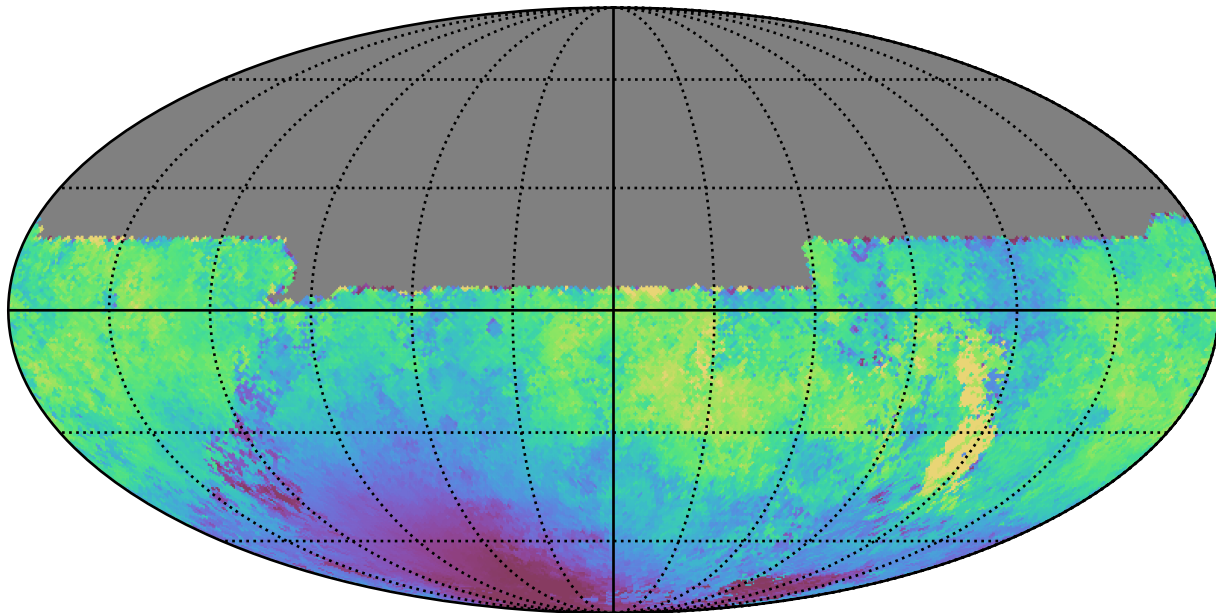
extra_ss_neo3_v3.4_10yrs All sky u band: Median moonDistance
