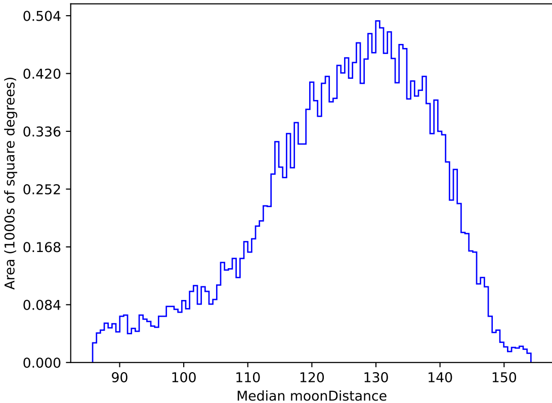
extra_ss_neo3_v3.4_10yrs All sky u band: Median moonDistance
