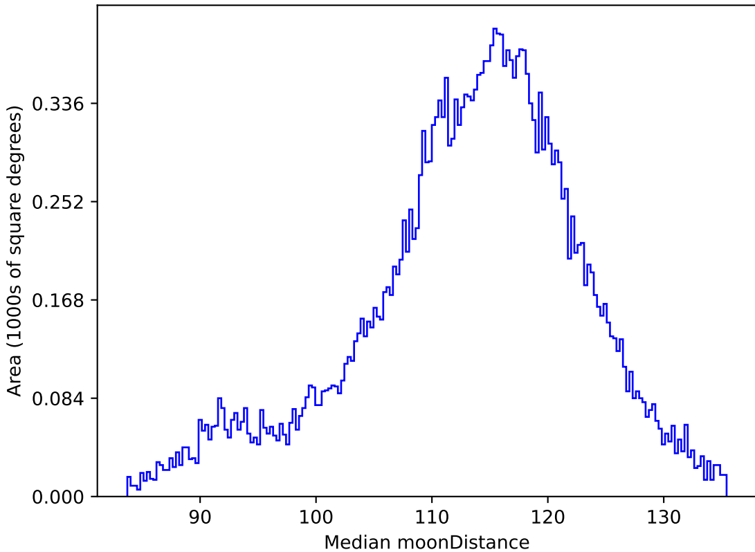
extra_ss_neo3_v3.4_10yrs All sky r band: Median moonDistance
