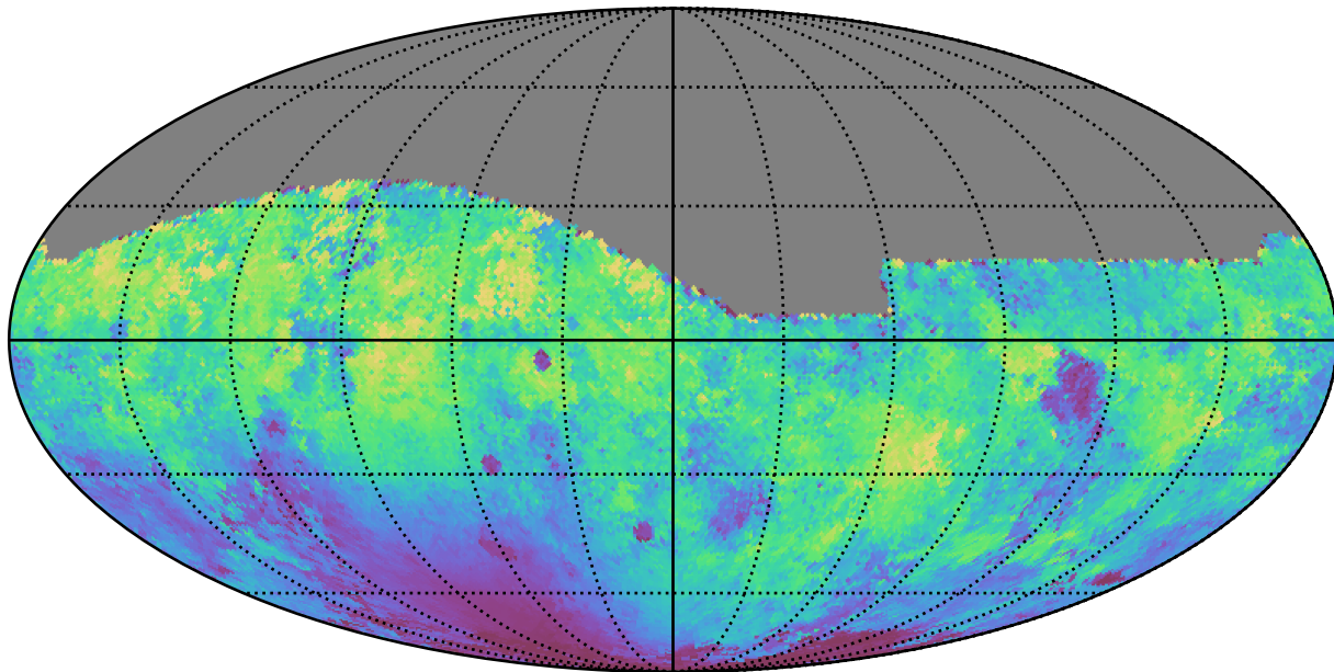
extra_ss_neo3_v3.4_10yrs All sky g band: Median moonDistance
