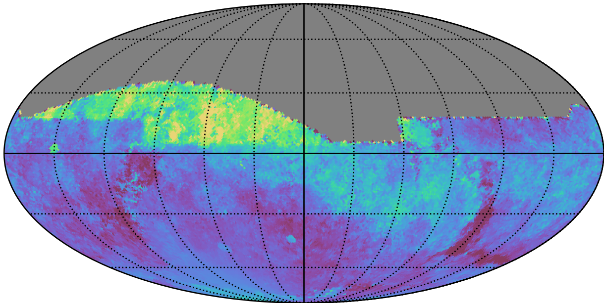
extra_ss_neo3_v3.4_10yrs All sky all bands: Median moonDistance
