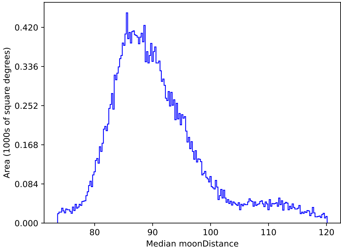
extra_ss_neo3_v3.4_10yrs All sky all bands: Median moonDistance
