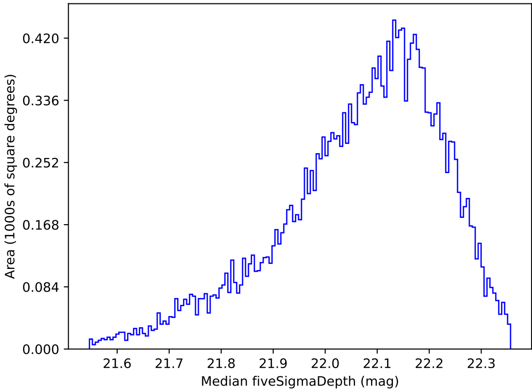
extra_ss_neo3_v3.4_10yrs Yr 1 y band: Median fiveSigmaDepth
