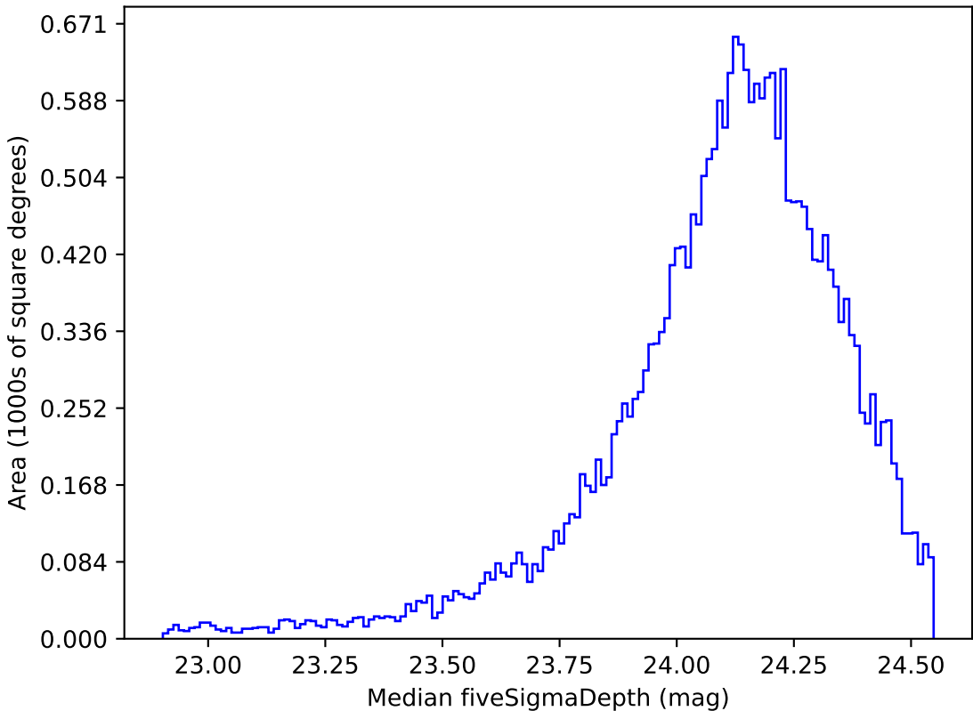
extra_ss_neo3_v3.4_10yrs Yr 1 r band: Median fiveSigmaDepth
