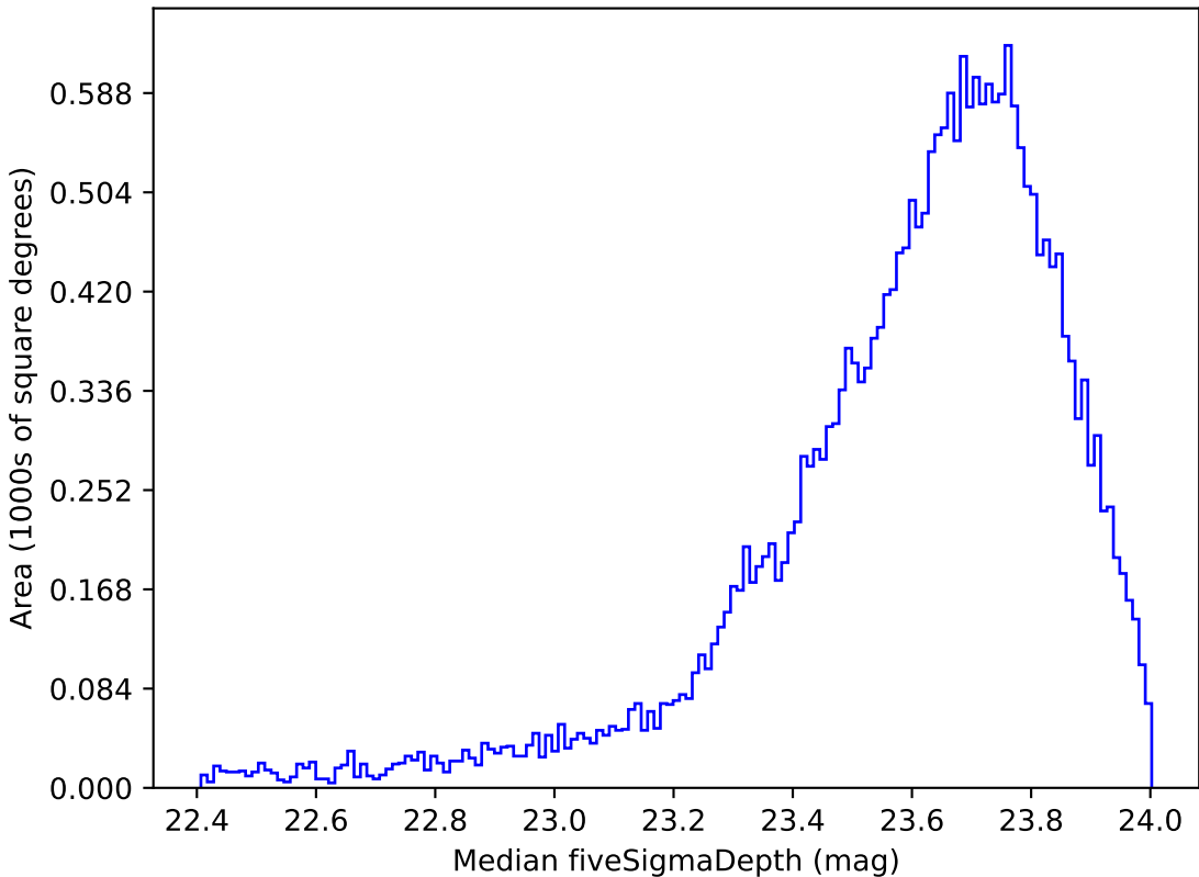
extra_ss_neo3_v3.4_10yrs Yr 1 i band: Median fiveSigmaDepth
