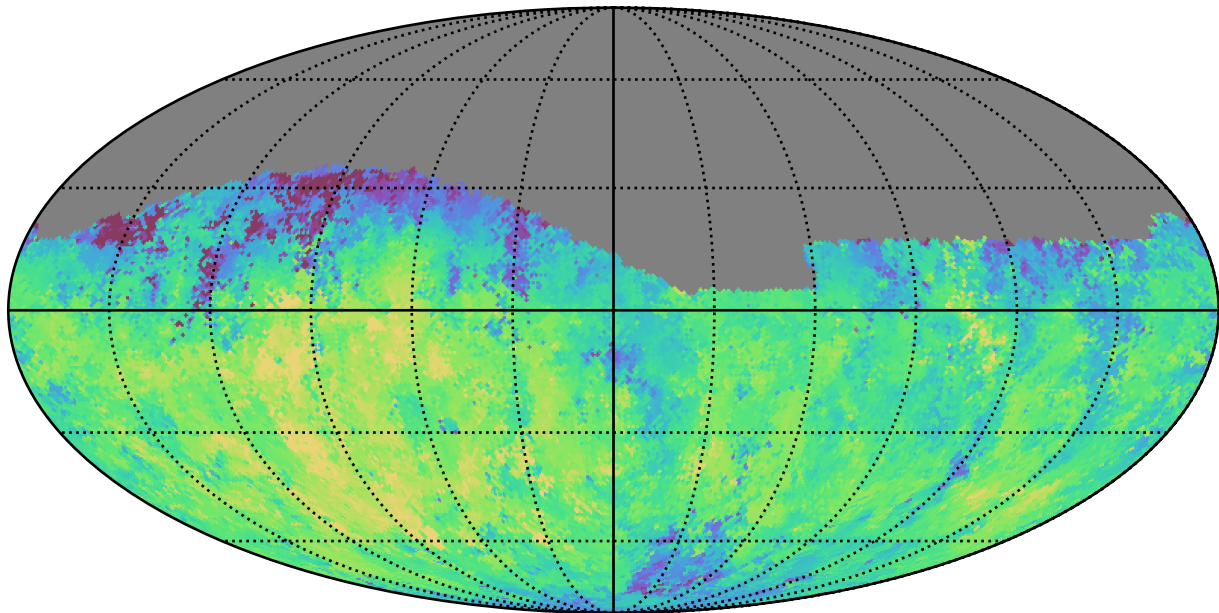
extra_ss_neo3_v3.4_10yrs Yr 1 g band: Median fiveSigmaDepth
