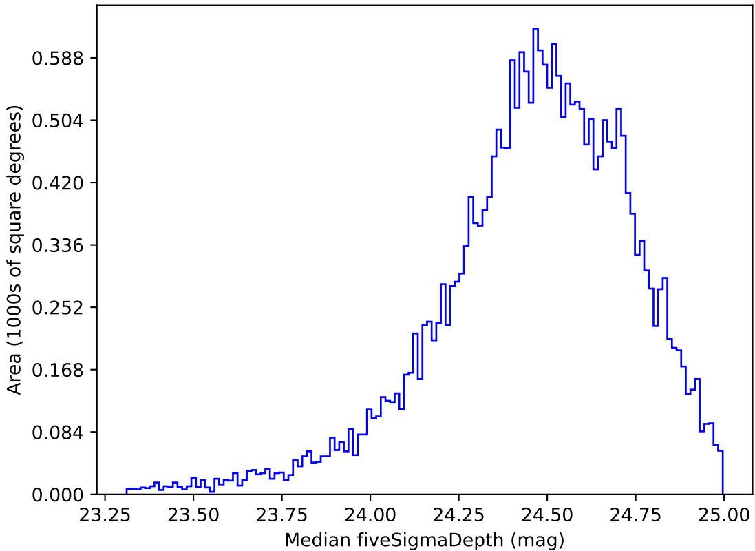
extra_ss_neo3_v3.4_10yrs Yr 1 g band: Median fiveSigmaDepth
