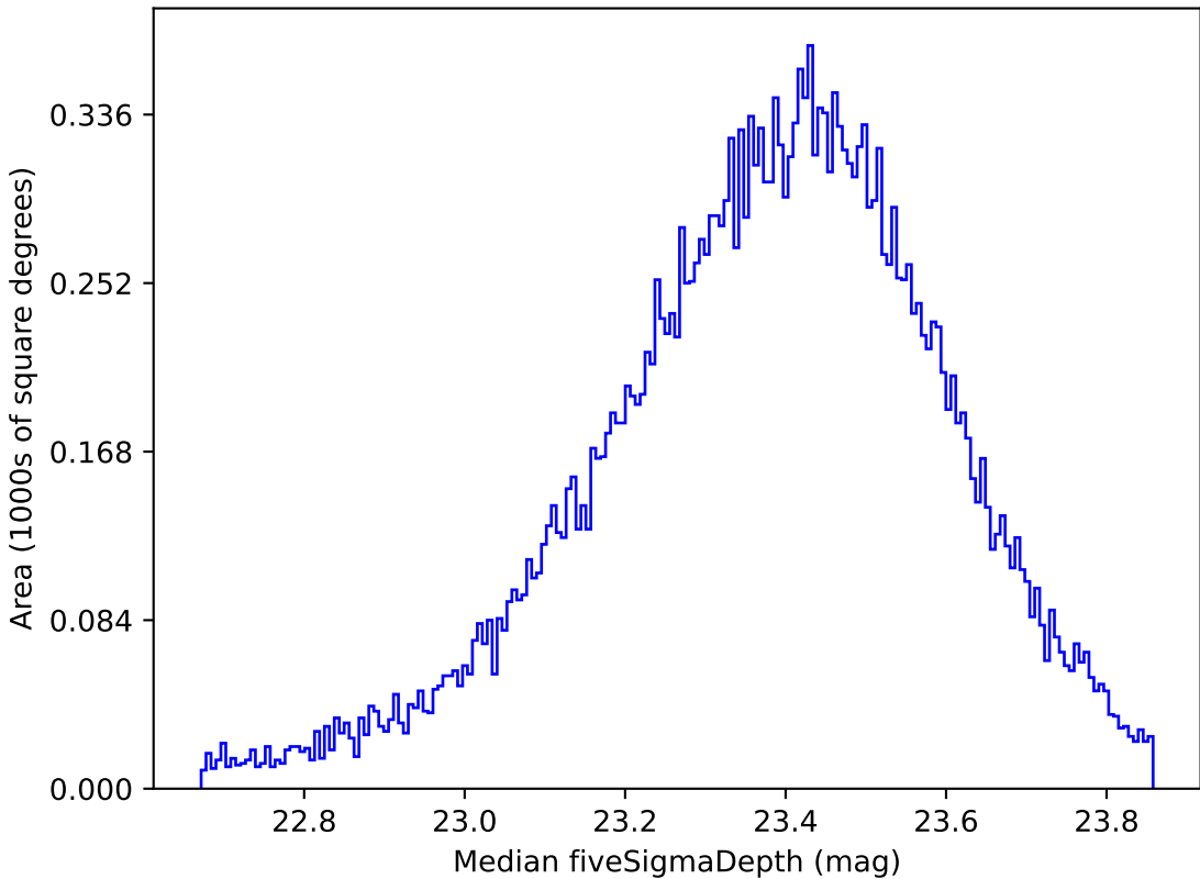
extra_ss_neo3_v3.4_10yrs Yr 1 all bands: Median fiveSigmaDepth
