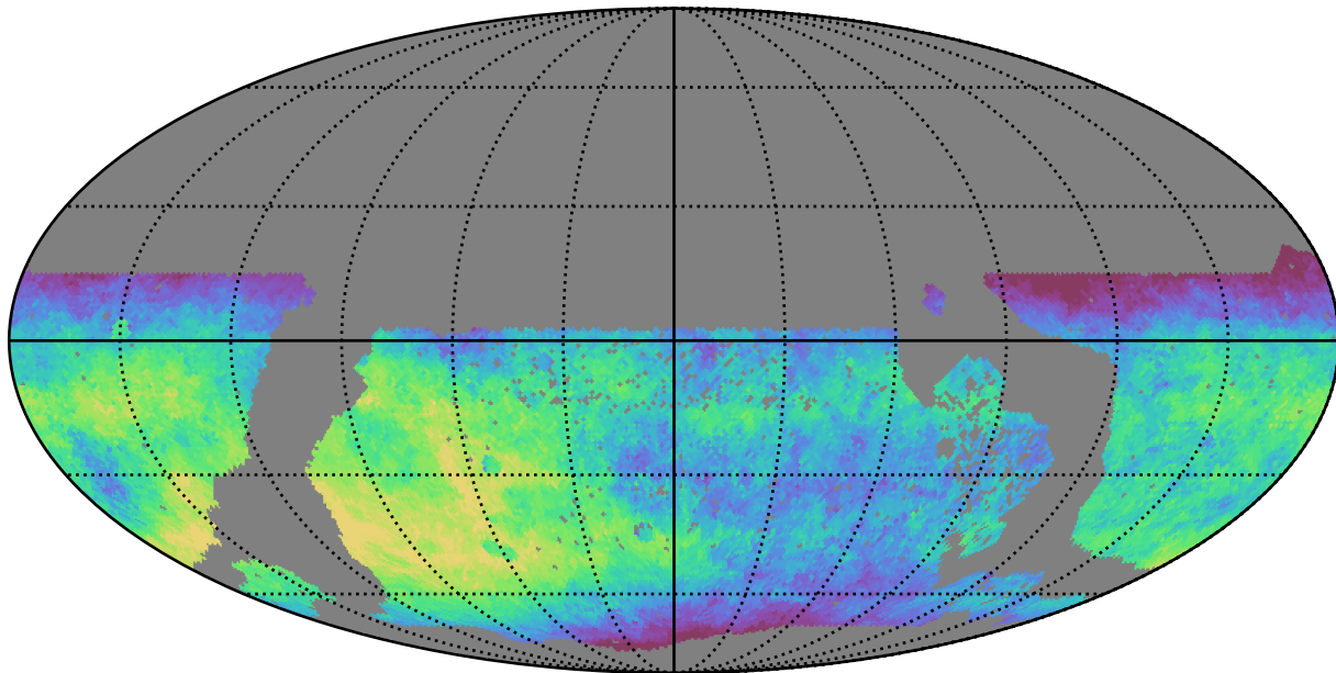
extra_ss_neo3_v3.4_10yrs WFD z band: Median fiveSigmaDepth
