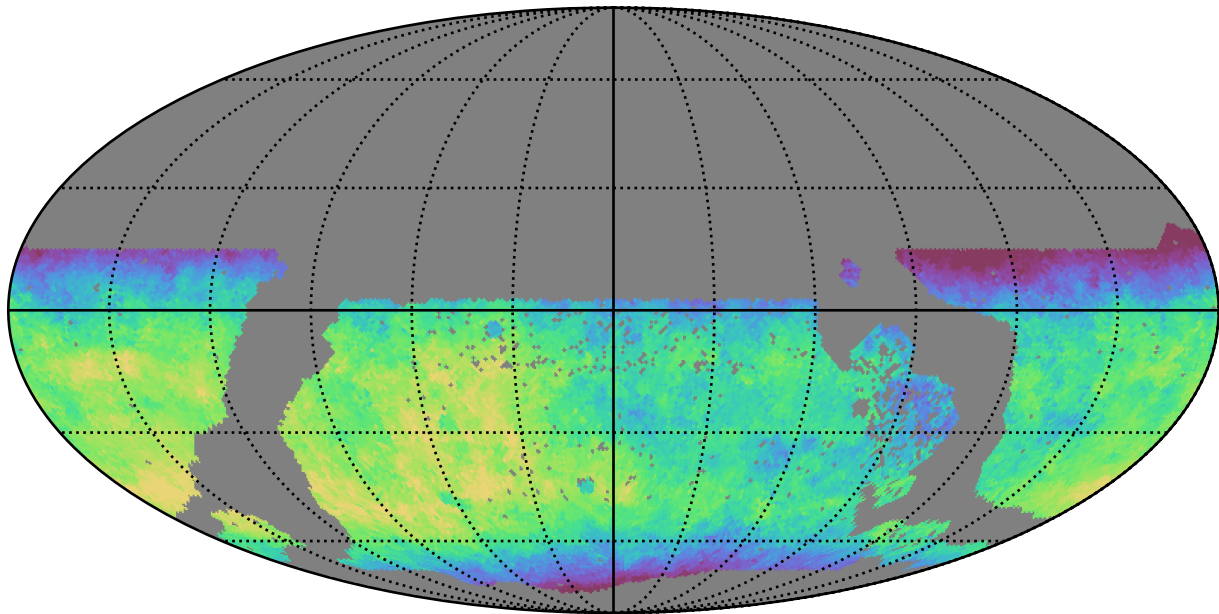
extra_ss_neo3_v3.4_10yrs WFD y band: Median fiveSigmaDepth
