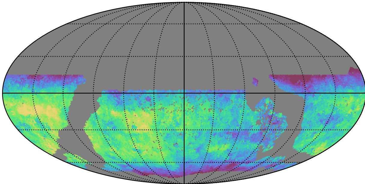
extra_ss_neo3_v3.4_10yrs WFD u band: Median fiveSigmaDepth
