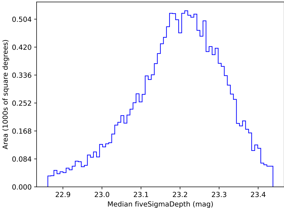
extra_ss_neo3_v3.4_10yrs WFD u band: Median fiveSigmaDepth
