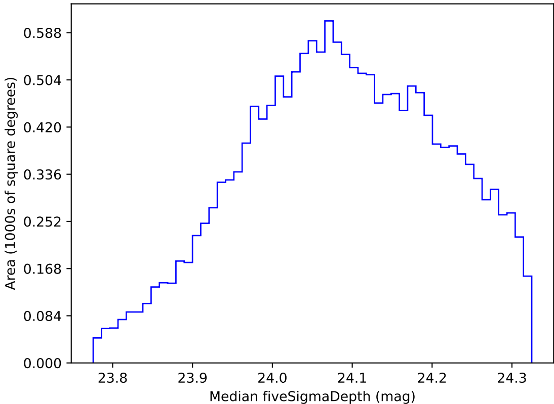
extra_ss_neo3_v3.4_10yrs WFD r band: Median fiveSigmaDepth
