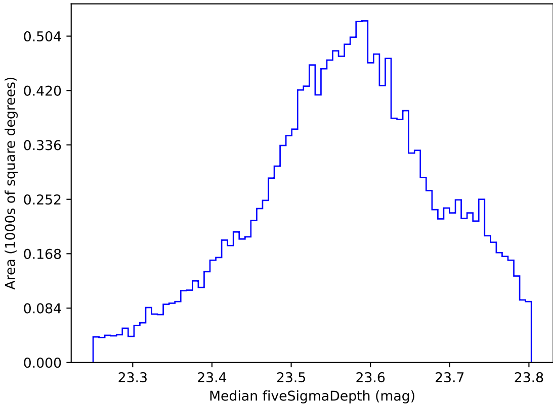
extra_ss_neo3_v3.4_10yrs WFD i band: Median fiveSigmaDepth
