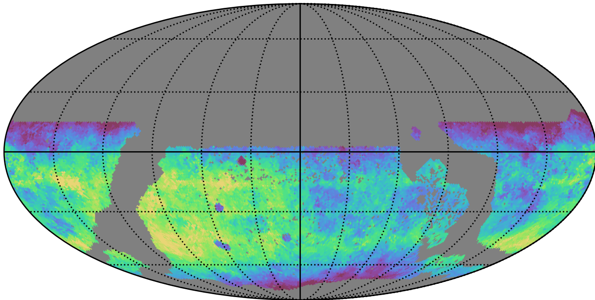
extra_ss_neo3_v3.4_10yrs WFD g band: Median fiveSigmaDepth
