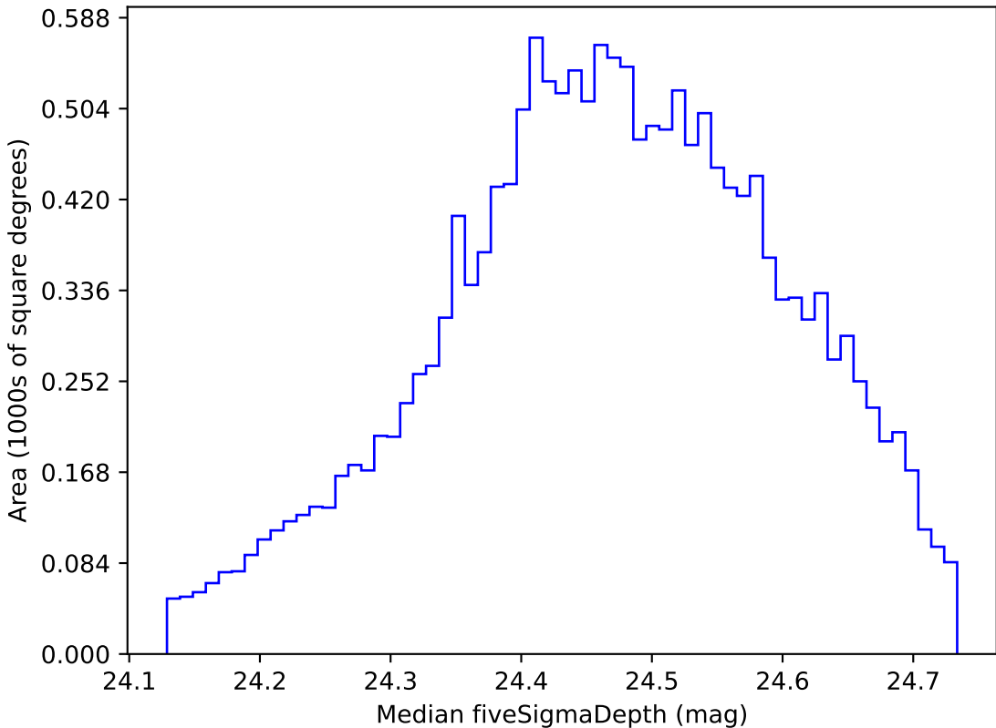
extra_ss_neo3_v3.4_10yrs WFD g band: Median fiveSigmaDepth
