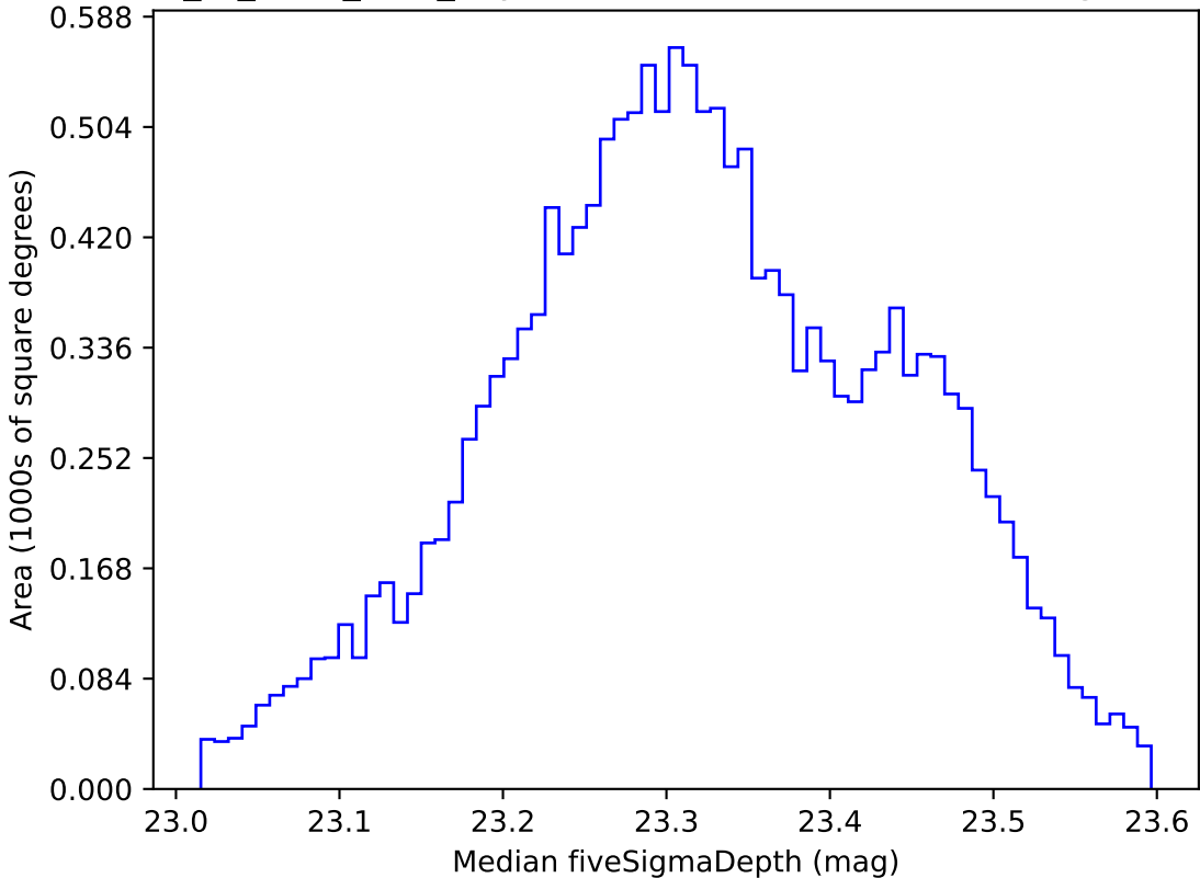
extra_ss_neo3_v3.4_10yrs WFD all bands: Median fiveSigmaDepth
