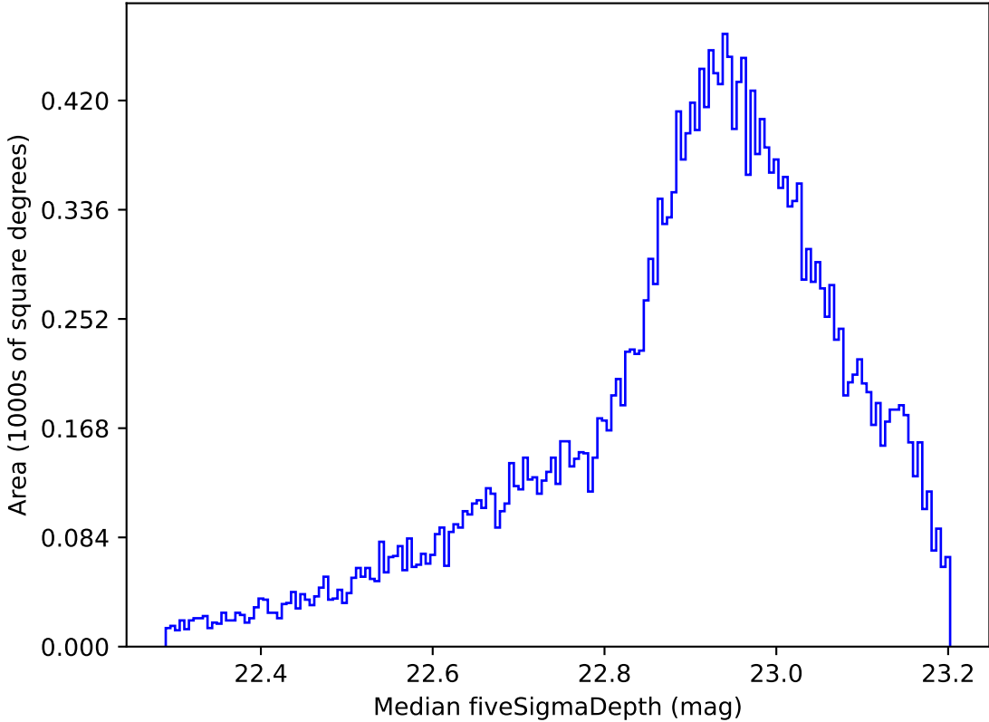
extra_ss_neo3_v3.4_10yrs All sky z band: Median fiveSigmaDepth
