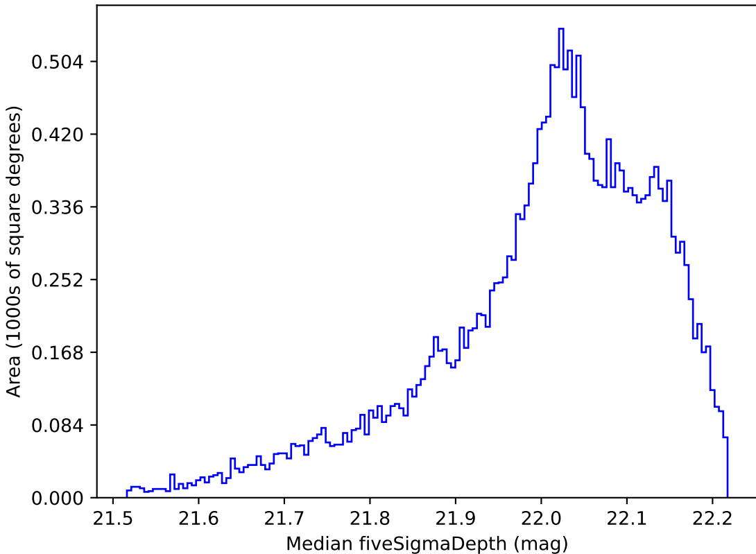
extra_ss_neo3_v3.4_10yrs All sky y band: Median fiveSigmaDepth
