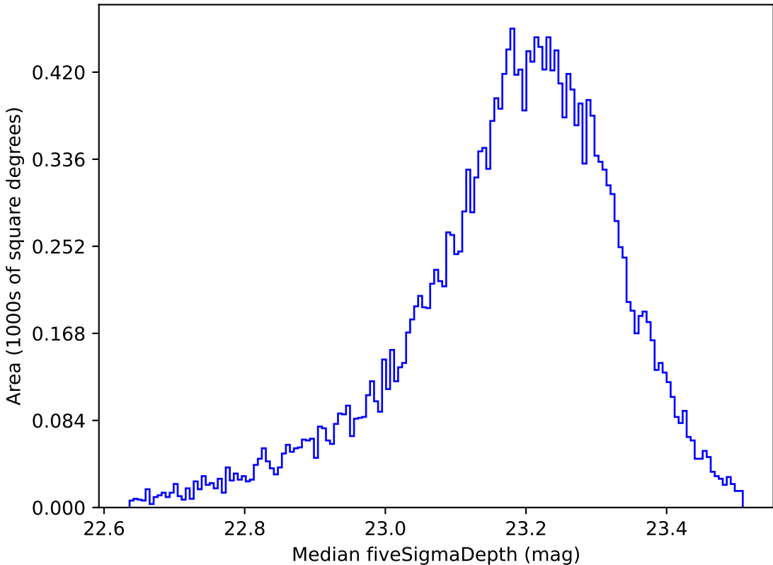
extra_ss_neo3_v3.4_10yrs All sky u band: Median fiveSigmaDepth
