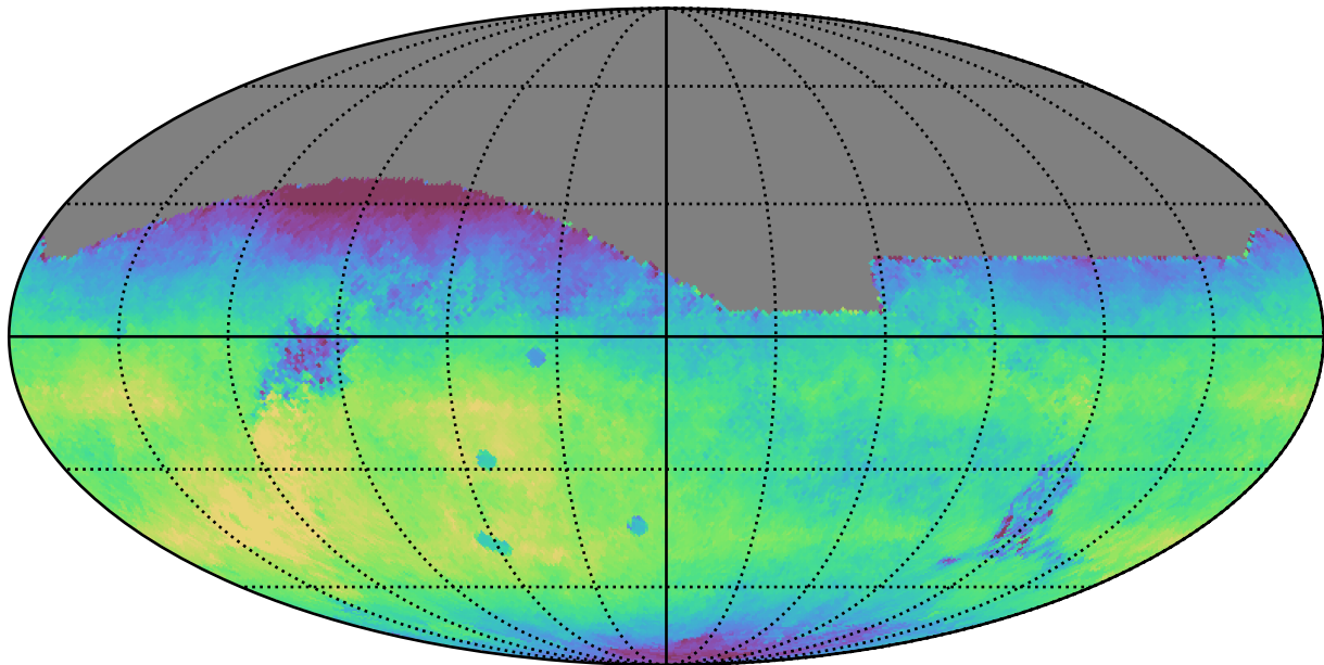
extra_ss_neo3_v3.4_10yrs All sky r band: Median fiveSigmaDepth
