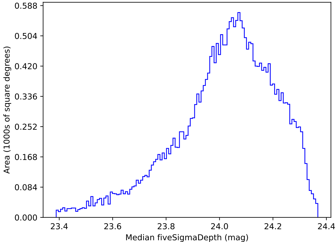
extra_ss_neo3_v3.4_10yrs All sky r band: Median fiveSigmaDepth
