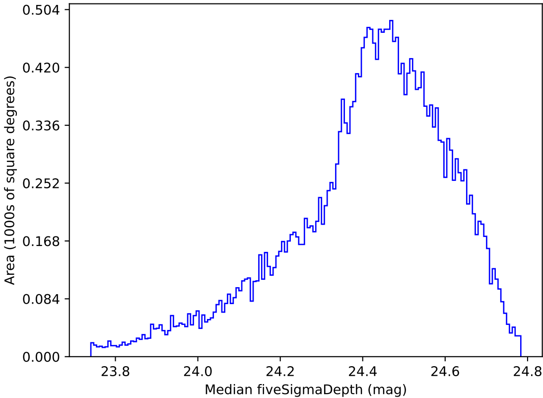
extra_ss_neo3_v3.4_10yrs All sky g band: Median fiveSigmaDepth
