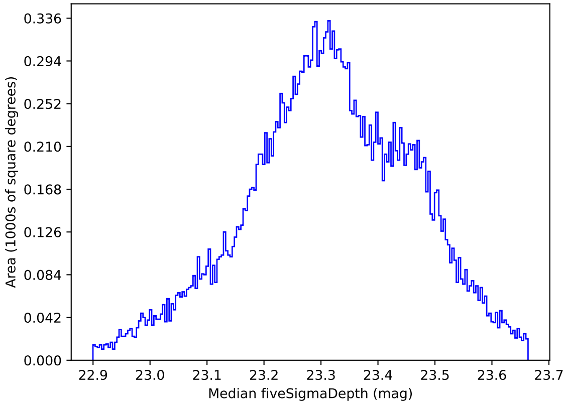
extra_ss_neo3_v3.4_10yrs All sky all bands: Median fiveSigmaDepth
