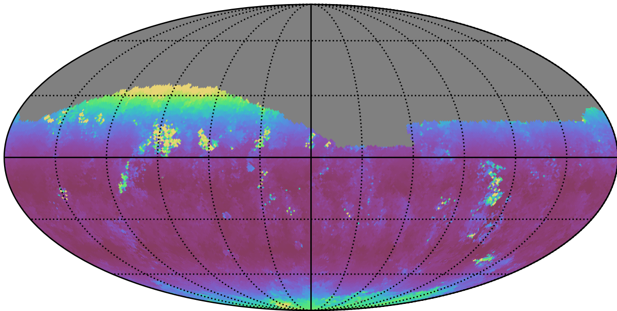
extra_ss_neo3_v3.4_10yrs Yr 1 z band: Median airmass
