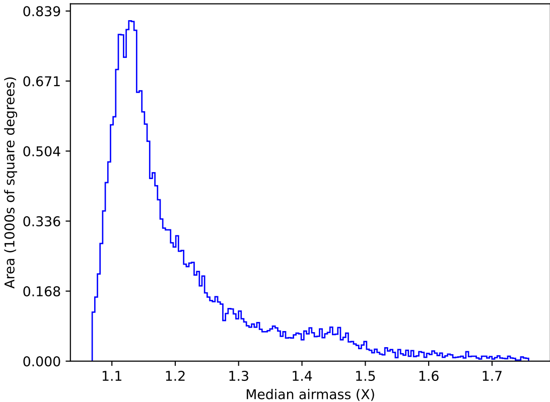
extra_ss_neo3_v3.4_10yrs Yr 1 y band: Median airmass
